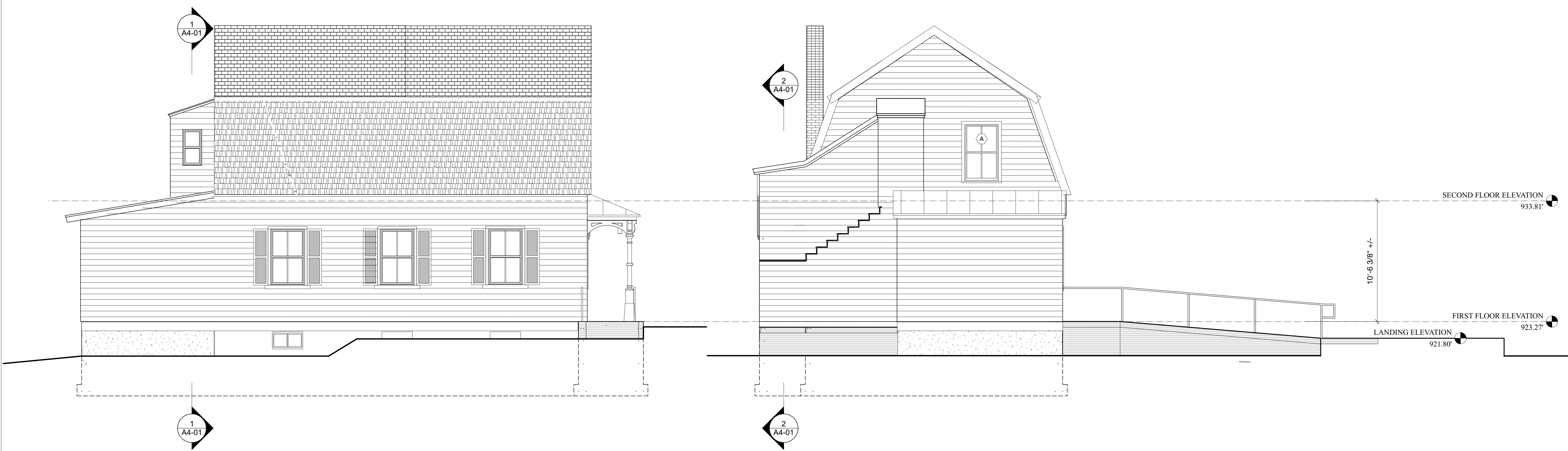
1 SOUTH ELEVATION 1/4" = 1'-0"
