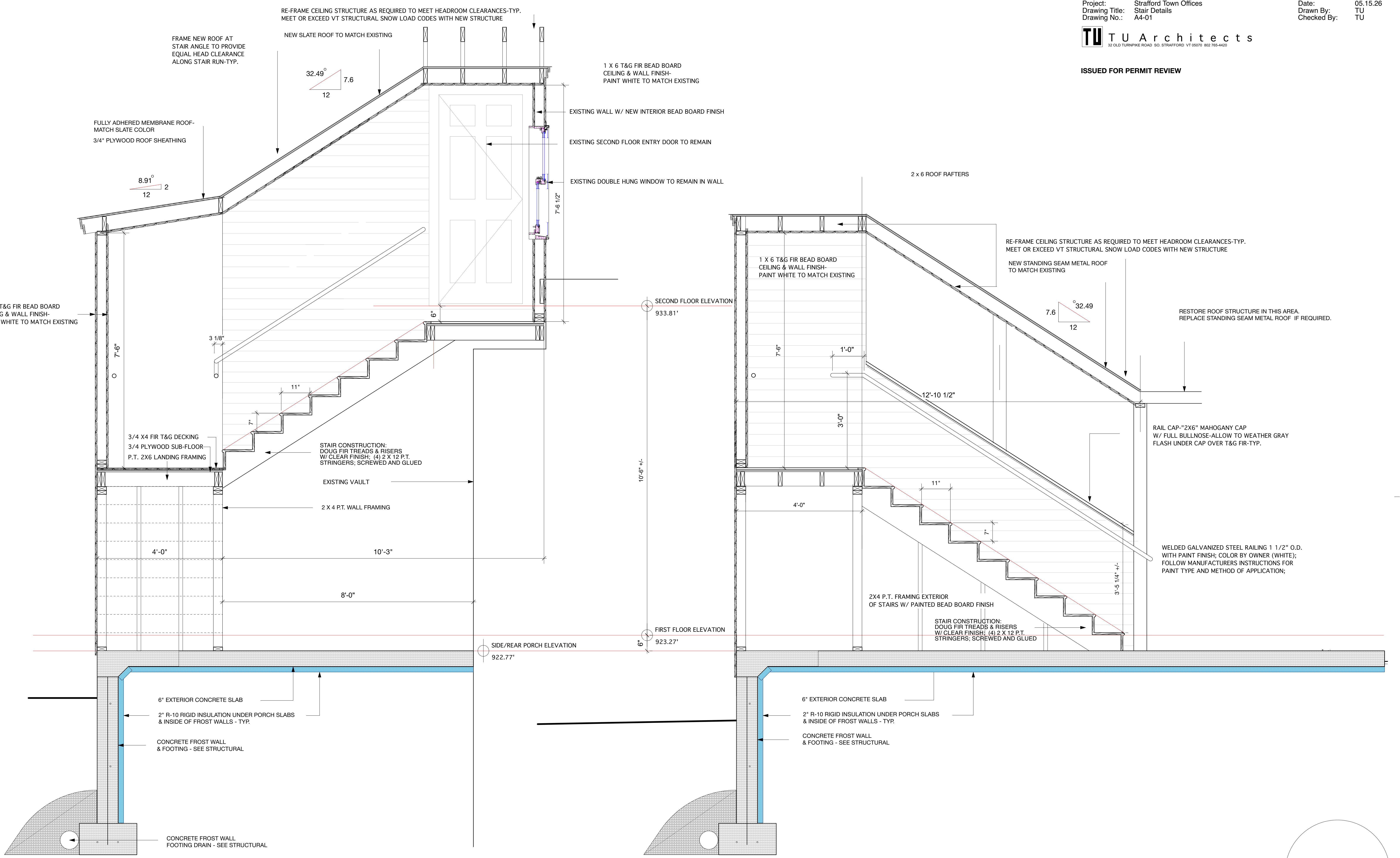
2. WALL SECTION ACROSS STAIR LANDING LOOKING NORTH 3/4" = 1'-0"
